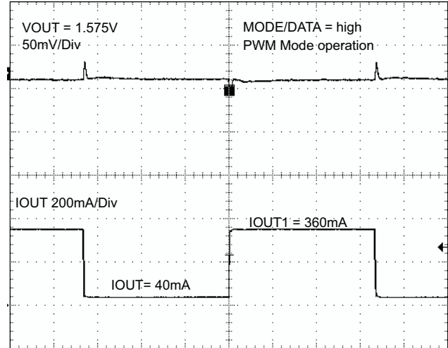
Time base - 50 \mu s/Div Figure 24.
