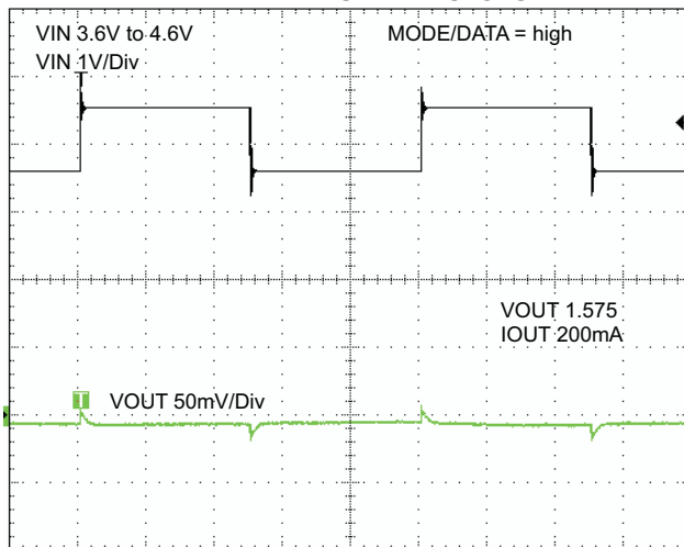
Time base - 400 \mu s/Div Figure 25.
