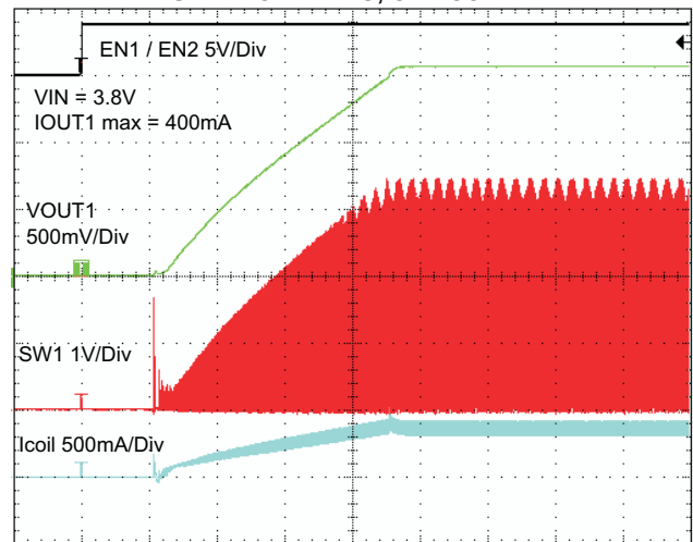
Time base - 200 \mu s/Div Figure 26.
