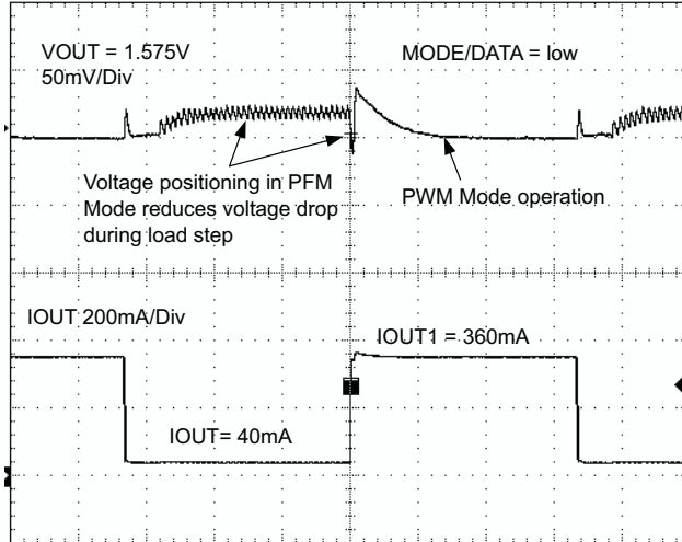
Time base - 50 \mu s/Div Figure 23.
