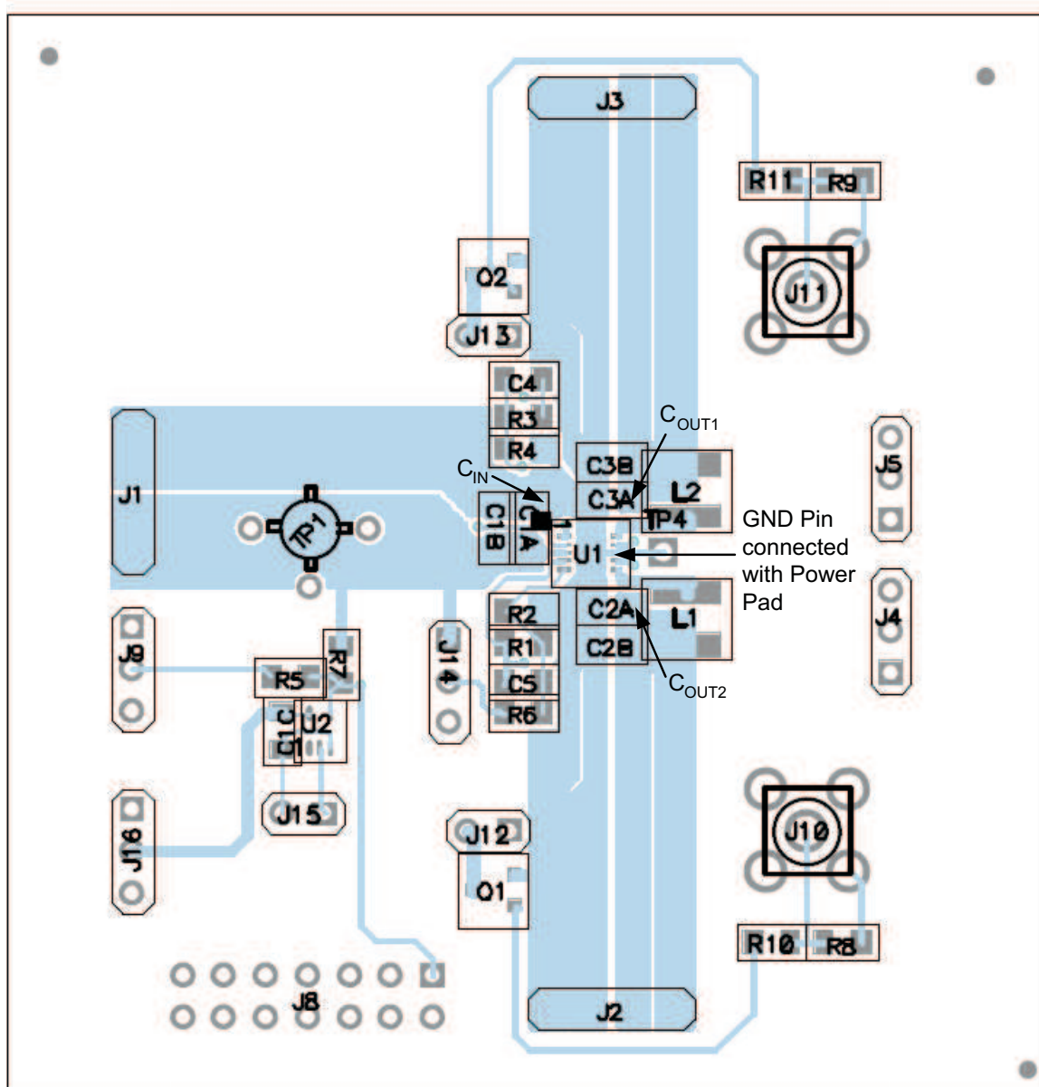
Figure 48. PCB Layout
