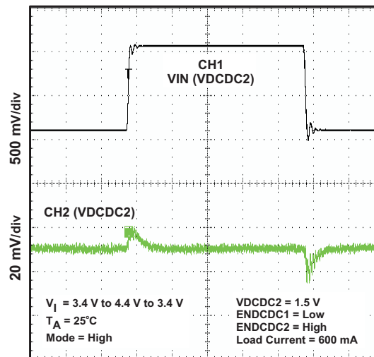
DCDC2 LINE TRANSIENT RESPONSE
