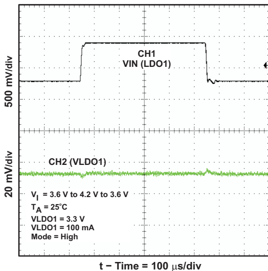
LDO1 LINE TRANSIENT RESPONSE
