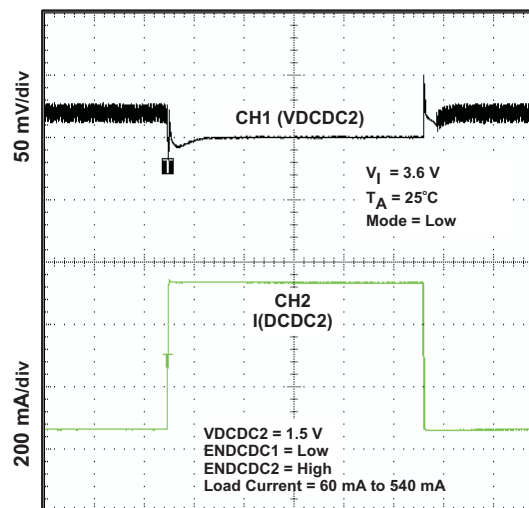
DCDC2 LOAD TRANSIENT RESPONSE
