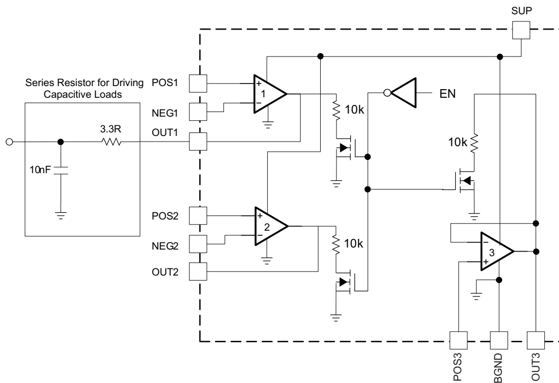
Figure 21. Operational Amplifier Block
