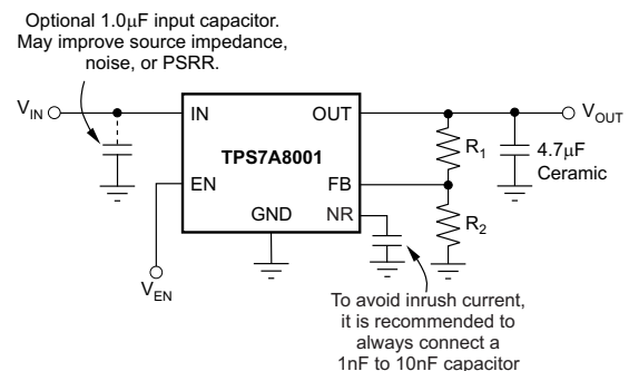
Typical Application Circuit for Adjustable Voltage Versions
