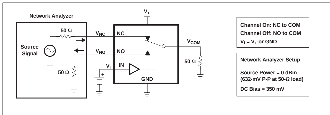
Figure 23. Crosstalk ( X_{TALK} )
