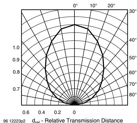
Fig. 4 - Horizontal Directivity
