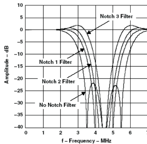
Figure 3-7. Chroma Trap Filter Frequency Response, PAL ITU-R BT.601 Sampling
