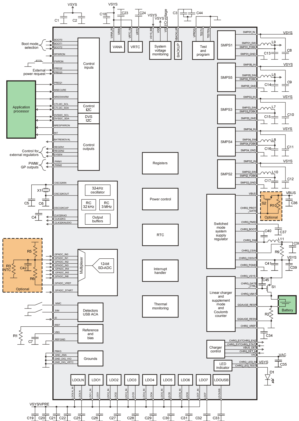
Figure 1. TWL6032 Device Block Diagram
