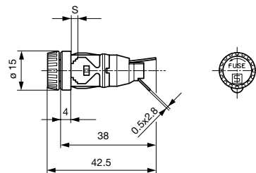
Variant Fingergrasp 0031.1913 and 0031.1914
