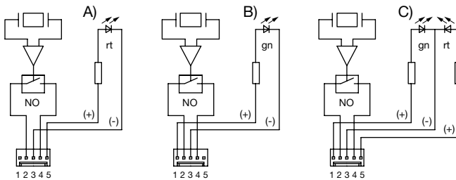
PSE M22 RI with Quick Connect Terminal, 12/24 V
