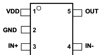
UCC27517 DBV (Top View)
