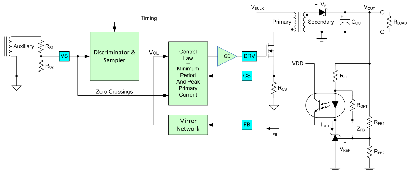
Figure 12. Simplified Flyback Convertor (With The Main Voltage Regulation Blocks)
