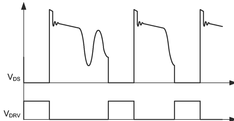
Figure 18. Valley-Skipping Mode
