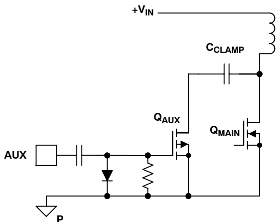
Figure 9. Low-Side P-Channel
