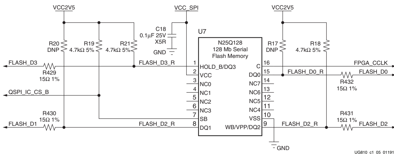
Figure 1-6: 128 Mb Quad-SPI Flash memory
