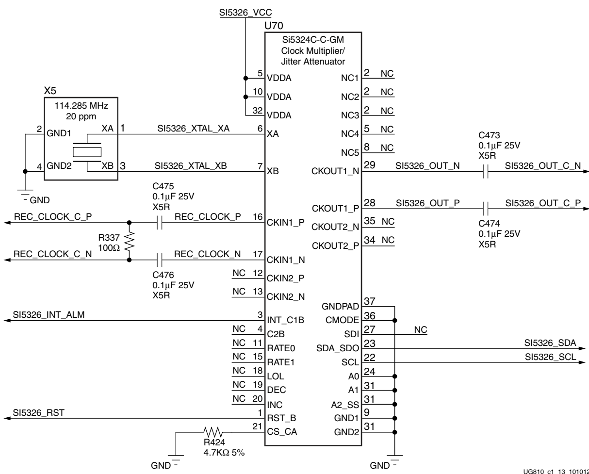
Figure 1-14: Jitter Attenuated Clock
