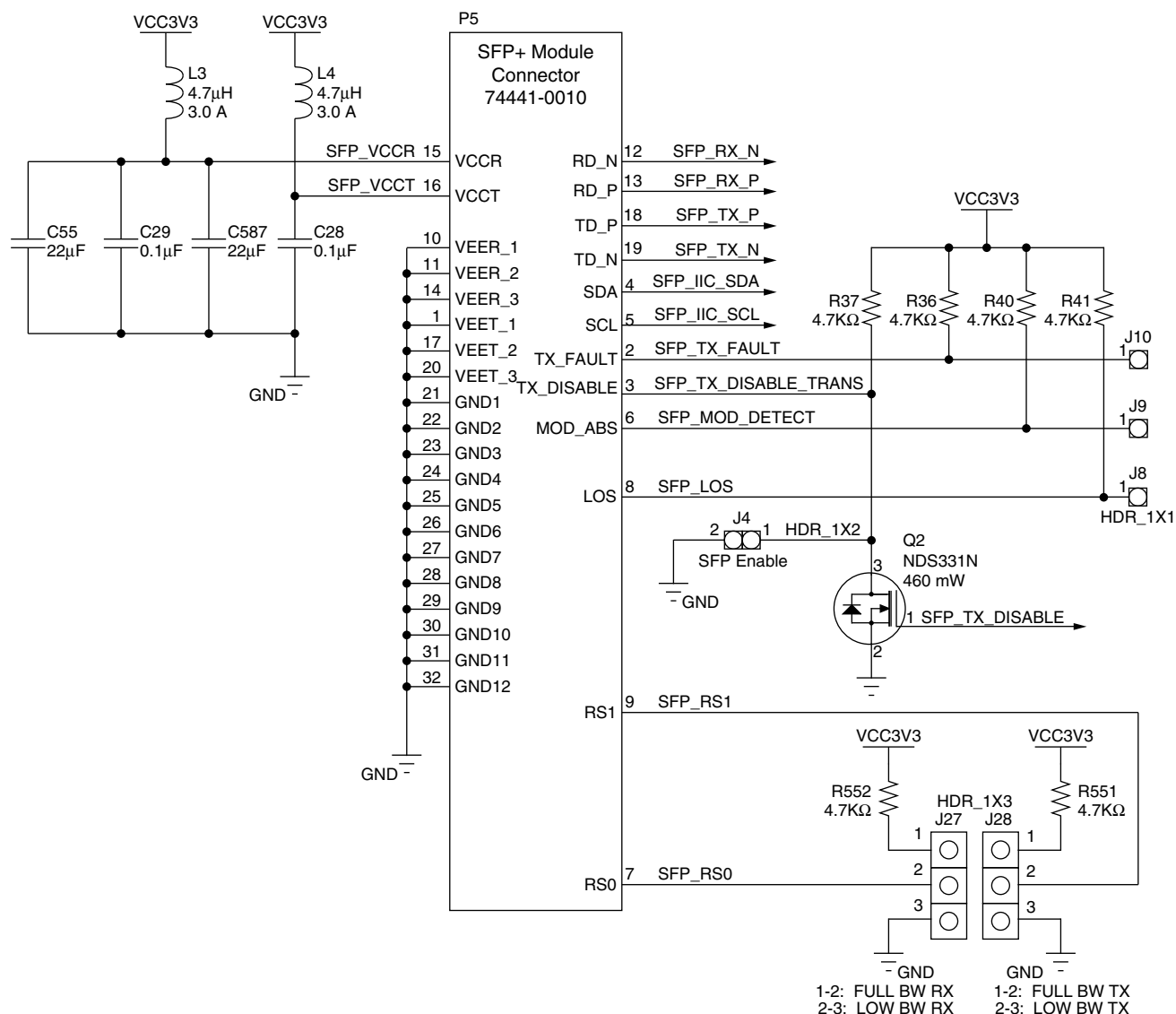
Figure 1-17: SFP+ Module Connector
