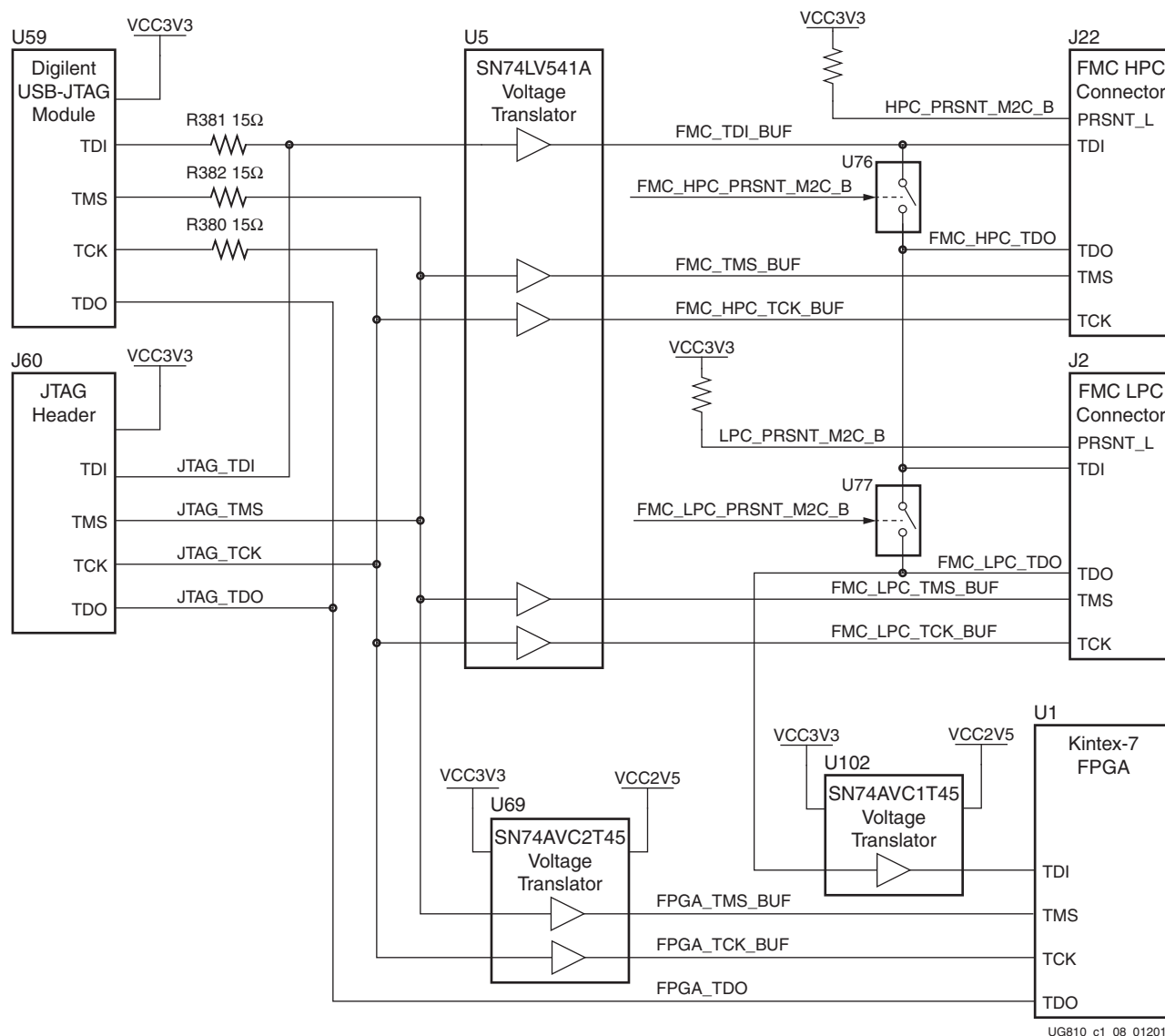
Figure 1-9: JTAG Circuit
