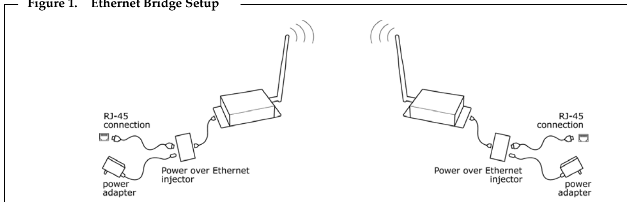
Figure 1. Ethernet Bridge Setup
