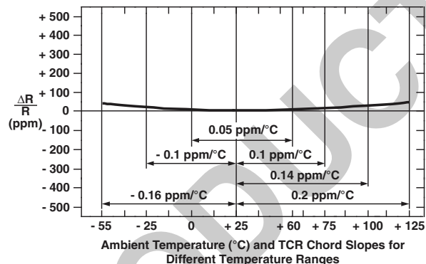
FIGURE 3 - TYPICAL RESISTANCE/TEMPERATURE CURVE
