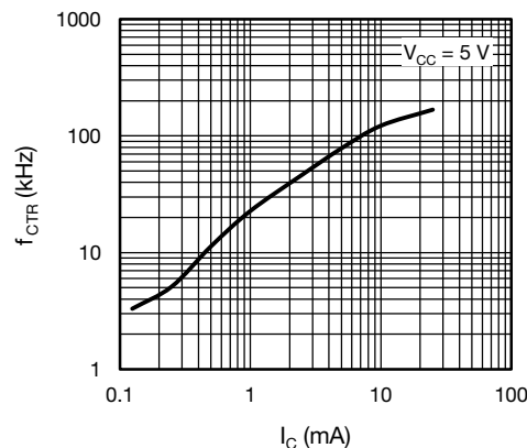
Fig. 15 - Cut-off Frequency ( -3\text{ dB} ) vs. Collector Current
