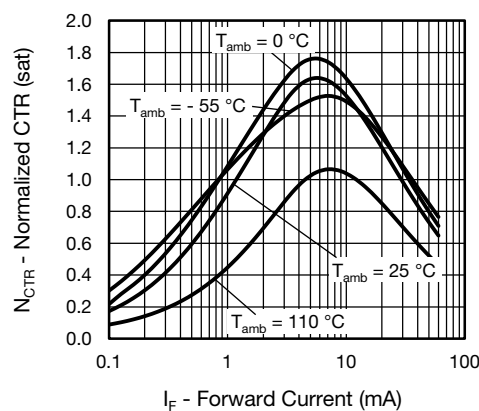
Fig. 13 - Current Transfer Ratio vs. Forward Current (non-saturated) Normalized to 1 mA at 25\text{ }^{\circ}C
