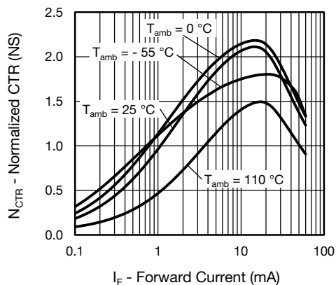
Fig. 12 - Current Transfer Ratio vs. Forward Current (saturated) Normalized to 1 mA at 25\text{ }^{\circ}C
