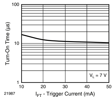
Fig. 7 - Trigger Current vs. Turn-On Time
