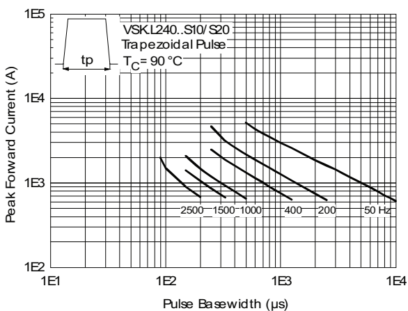
Fig. 23 - Frequency Characteristics
