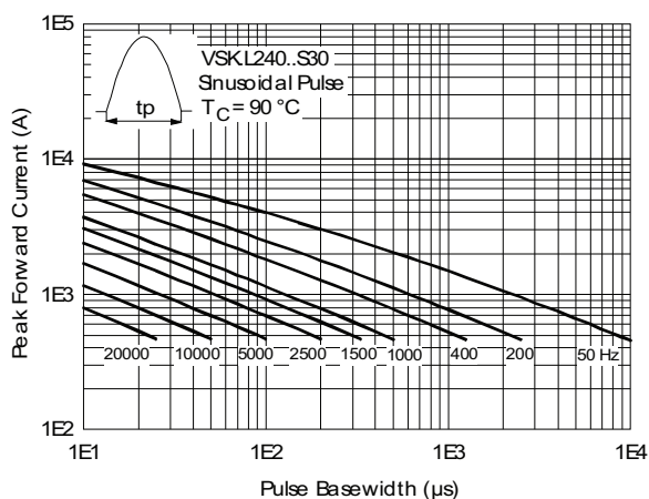
Fig. 25 - Frequency Characteristics
