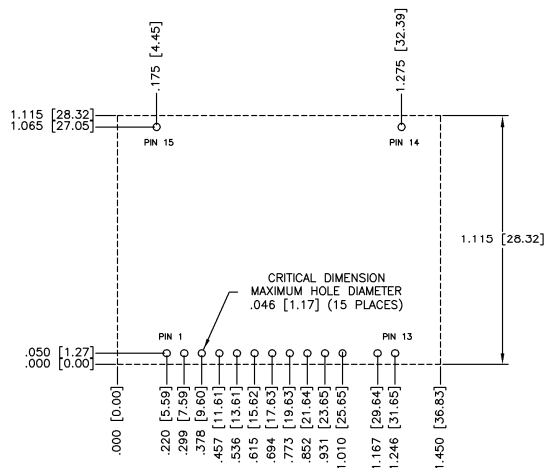
Figure 21. Mechanical Drawing
