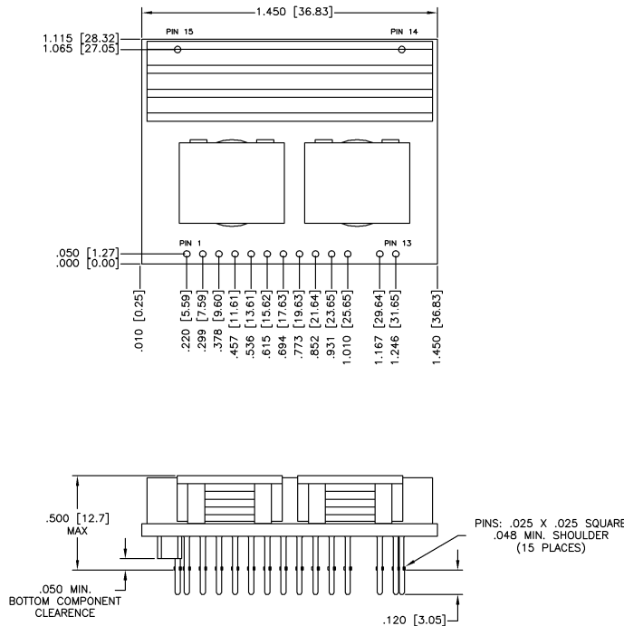
Figure 21. Mechanical Drawing
