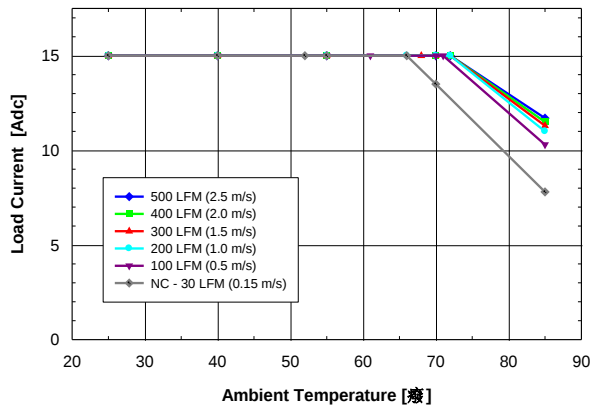
Figure 1. Available load current vs. ambient air temperature and airflow rates for SSQE48T15033 converter mounted vertically with air flowing from pin 1 to pin 3, V_{in} = 48\text{ V} . Note: NC – Natural convection
