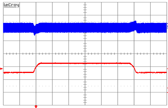
Figure 8. Output voltage response to load current step-change (7.5A–10.25A–7.5A) at V_{in}=48\text{V} . Top trace: output voltage (100 mV/div.). Bottom trace: load current (5A/div.). Current slew rate: 0.1A/ \mu\text{s} . C_o=1\mu\text{F} ceramic + 10 \mu\text{F} tantalum. Time scale: 0.2ms/div.
