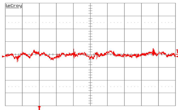
Figure 12. Input reflected-ripple current, i_s (10mA/div.), measured through 10\mu\text{H} at the source at full rated load current and V_{in} = 48\text{V} . Refer to Figure 11 for test setup. Time scale: 1\mu\text{s}/\text{div} .
