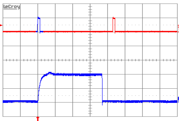
Figure 15. Load current (top trace, 20A/div., 50ms/div.) into a 10\text{m}\Omega short circuit during restart, at V_{in} = 48\text{V} . Bottom trace (10 A/div., 2 ms/div.) is an expansion of the on-time portion of the top trace
