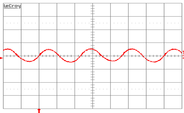
Figure 13. Input reflected ripple-current, i_c (200mA/div.), measured at input terminals at full rated load current and V_{in} = 48\text{V} . Refer to Figure 11 for test setup. Time scale: 1\mu\text{s}/\text{div} .
