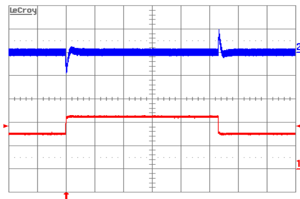
Figure 9. Output voltage response to load current step-change (7.5A –10.25A–7.5A) at V_{in}=48\text{V} . Top trace: output voltage (100 mV/div.). Bottom trace: load current (5A/div.). Current slew rate: 5A/ \mu\text{s} . C_o= 470\mu\text{F} POS + 1 \mu\text{F} ceramic. Time scale: 0.2 ms/div.
