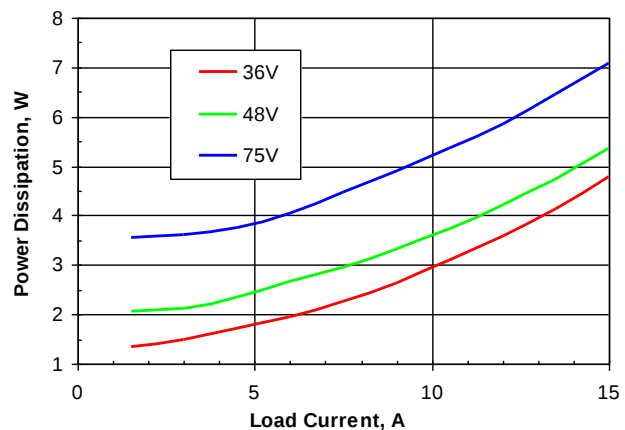
Figure 4. Power dissipation vs. load current and input voltage for SSQE48T15033 converter mounted vertically with air flowing from pin 1 to pin 3 at a rate of 300 LFM (1.5 m/s) and T_a = 25^\circ\text{C}
