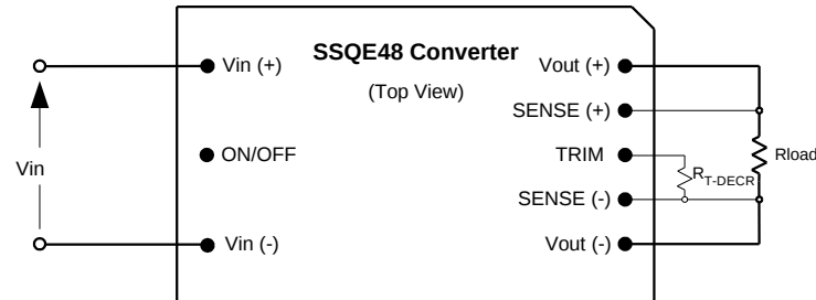
Fig. D: Configuration for decreasing output voltage.
