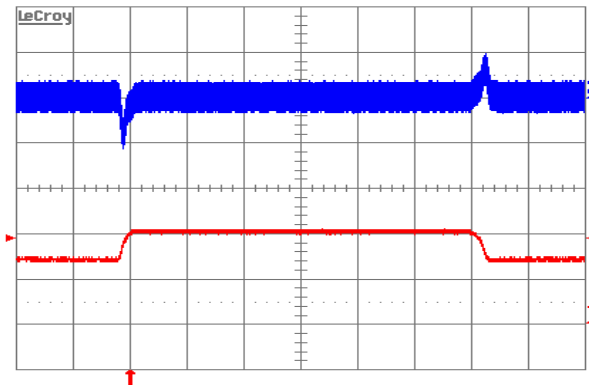
Figure 8. Output voltage response to load current step-change (6.5A–9.75A–6.5A) at V_{\text{in}}=48\text{V} . Top trace: output voltage (100 mV/div.). Bottom trace: load current (5A/div.). Current slew rate: 0.1A/ \mu\text{s} . C_o=1\mu\text{F} ceramic + 10 \mu\text{F} tantalum. Time scale: 0.2ms/div.
