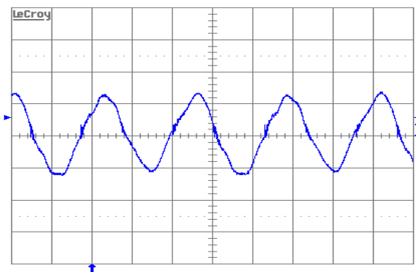
Figure 10. Output voltage ripple (20 mV/div.) at full rated load current into a resistive load with C_o = 10 \mu\text{F} tantalum + 1 \mu\text{F} ceramic and V_{\text{in}} = 48 \text{ V} . Time scale: 1 \mu\text{s}/\text{div} .
