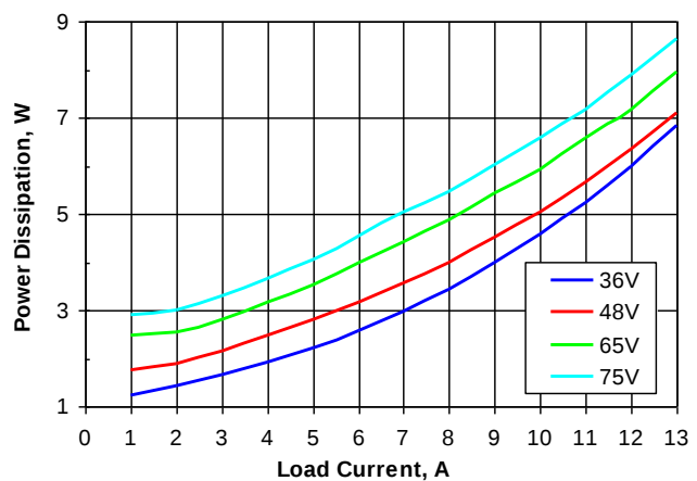
Figure 4. Power dissipation vs. load current and input voltage for SSQE48T13050 converter mounted vertically with air flowing from pin 1 to pin 3 at a rate of 300 LFM (1.5 m/s) and T_a = 25\text{ °C}
